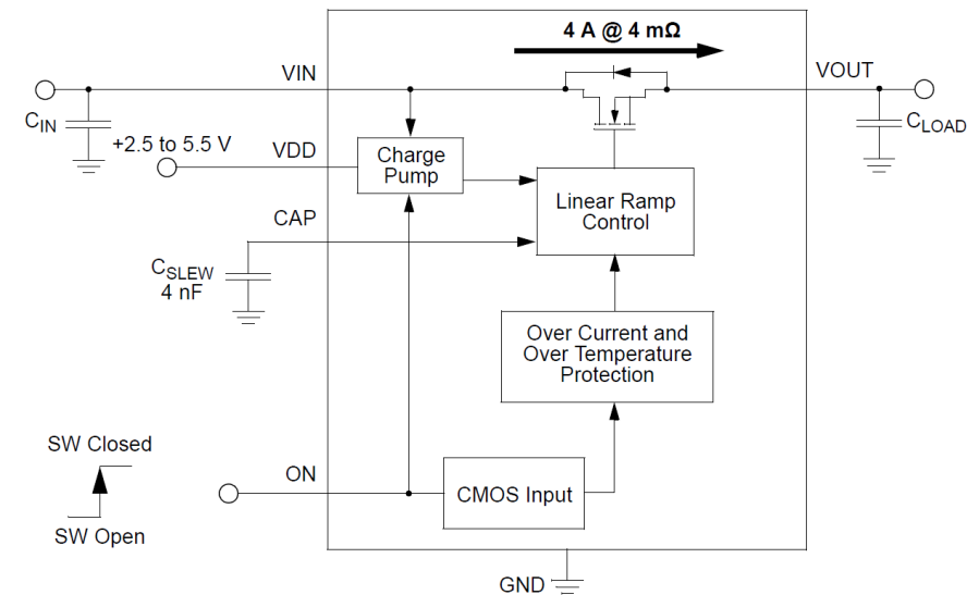
Figure 1: SLG59M1709V Block Diagram
