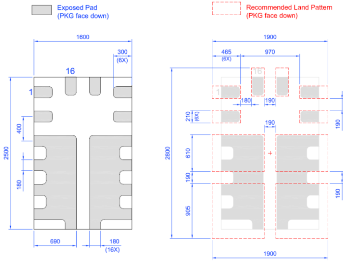
Figure 2. SLG59M1709V Package Dimensions and Recommended Land Pattern
