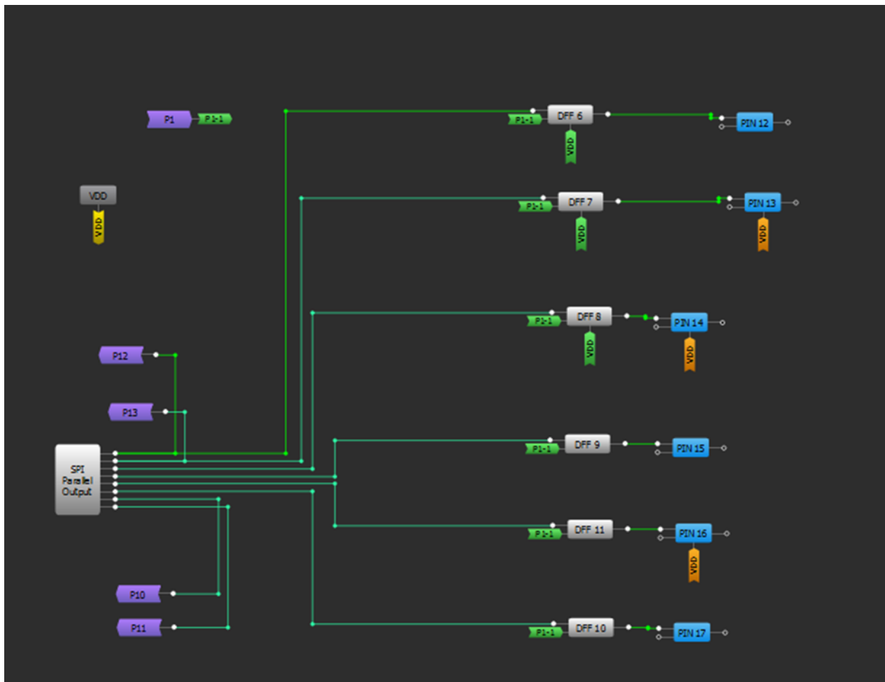
Figure 5. SPI Parallel Output Block Pins
