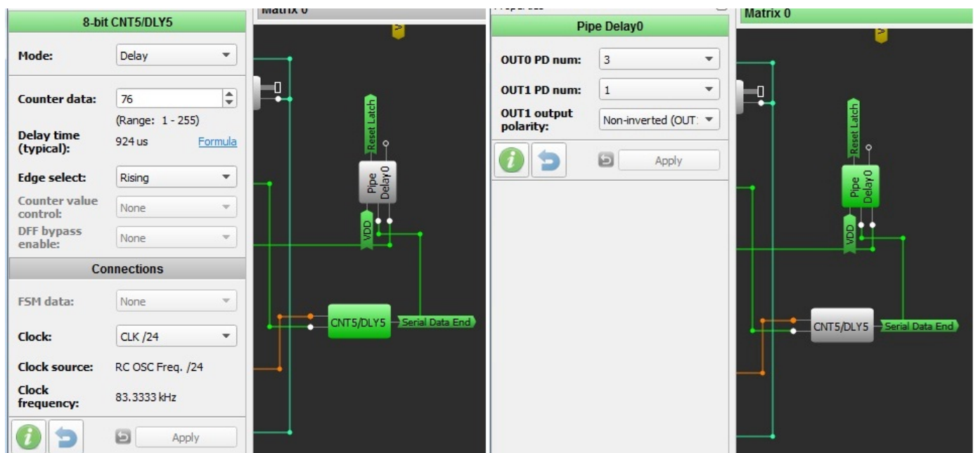
Figure 4. CNT5/DLY5 and Pipe Delay 0 properties
