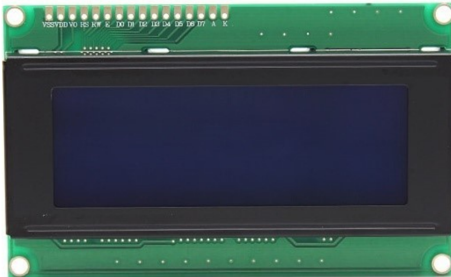
Figure 7. LCD 2004A Photo
