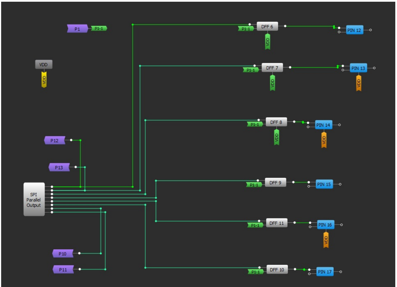
Figure 5. SPI Parallel Output Block Pins
