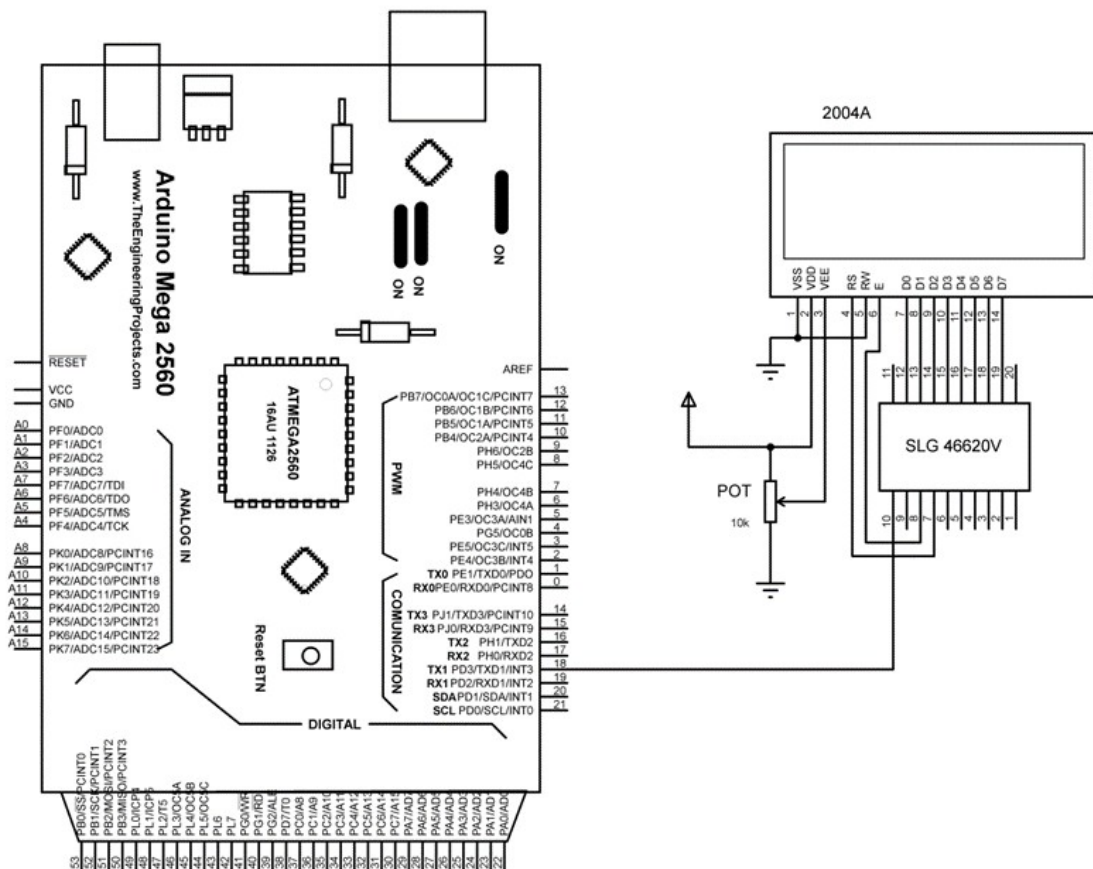
Figure 1. SLG46620V GreenPAK4 CMIC
