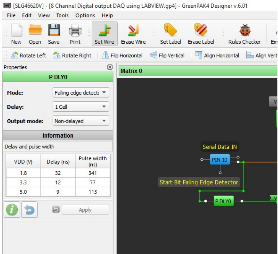
Figure 3. P DLY0 block Properties
