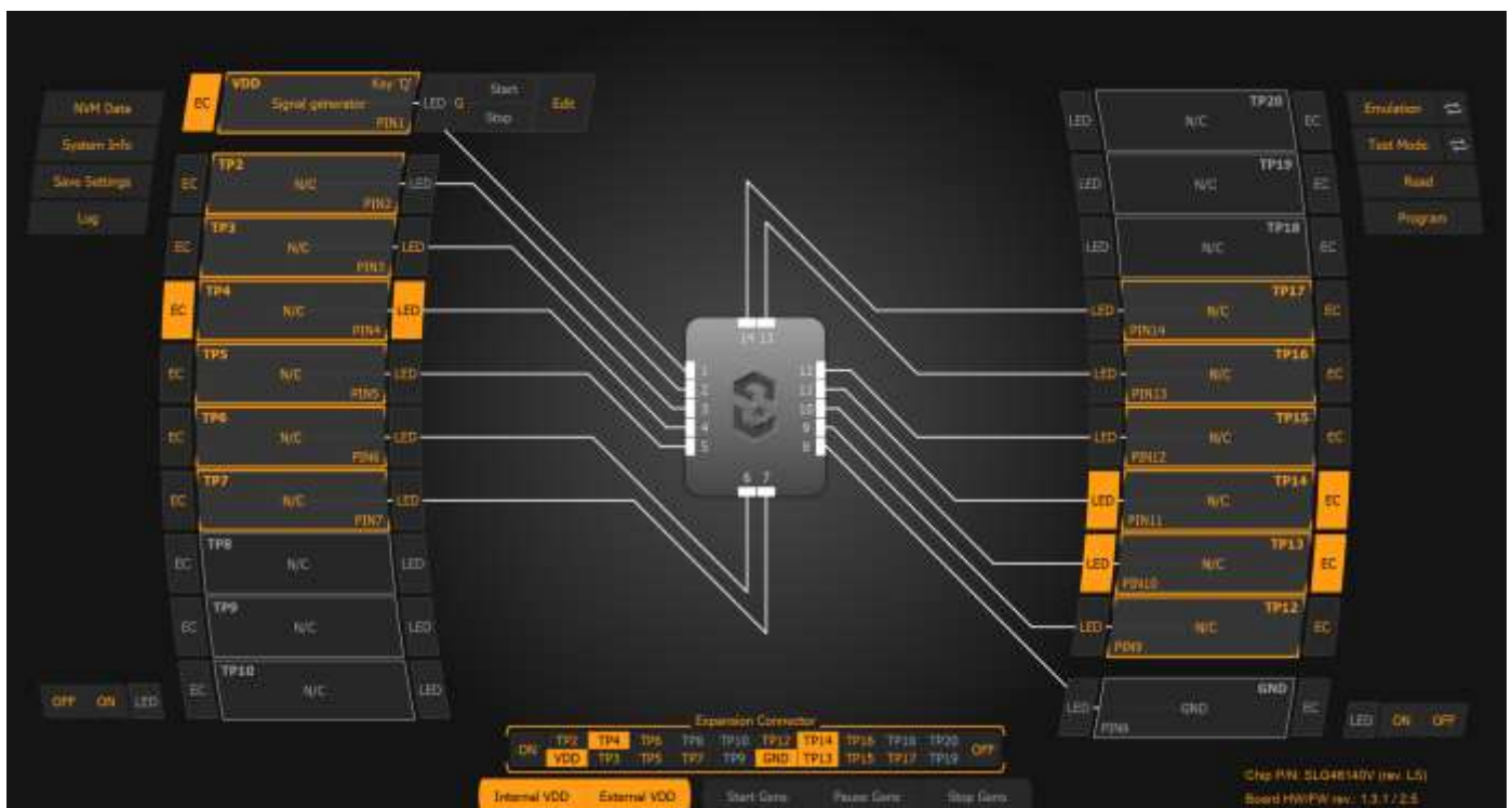
Figure 16. The GreenPAK Designer emulation window used to test the CO detector system
