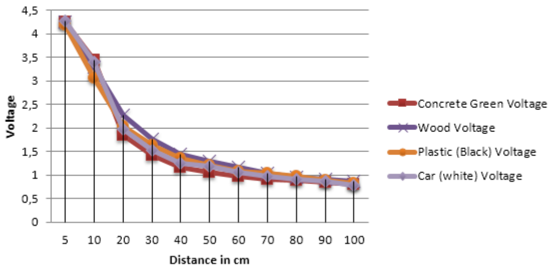
Figure 5. Voltage graph
